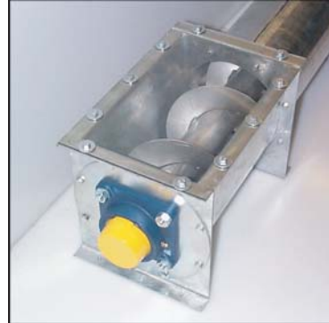
Outlet & drive section on 160mm conveyor
