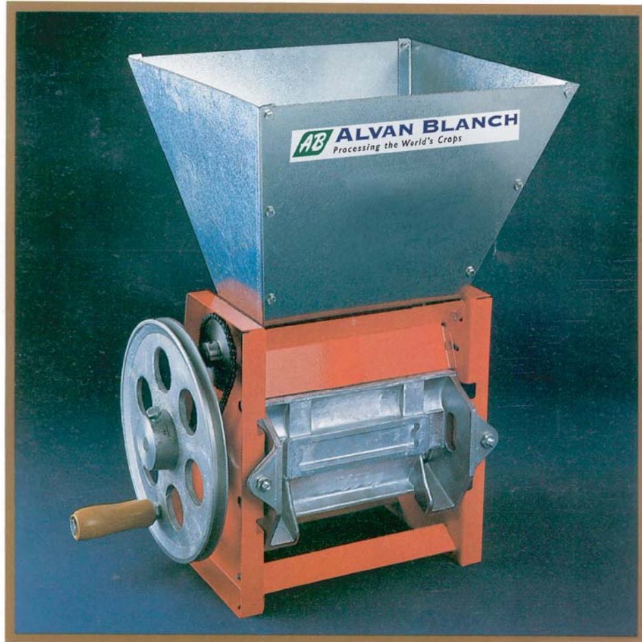
Drum Pulper
